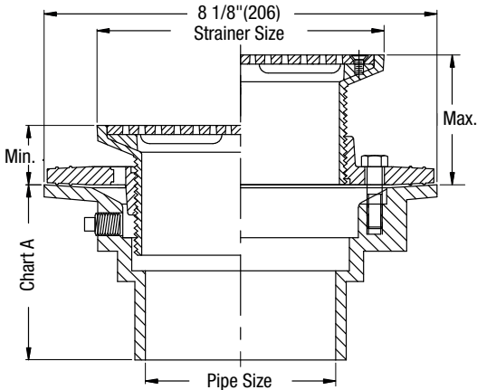
Strainer Size
