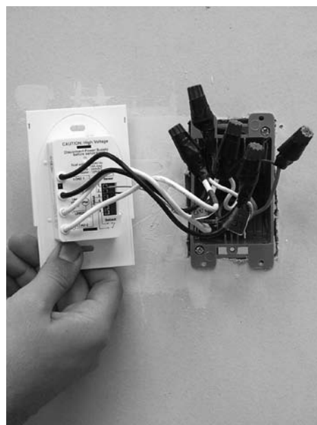
The mat power leads and sensor wire connected to the control at the electrical box.
