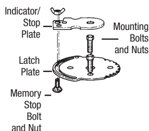
Positioning/Locking Kit
