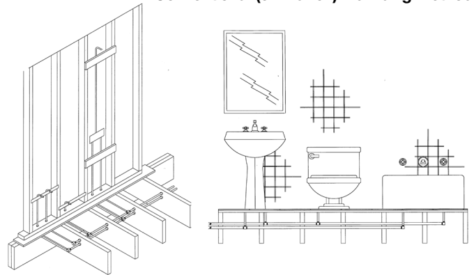
Conventional (or Branch) Plumbing Method
