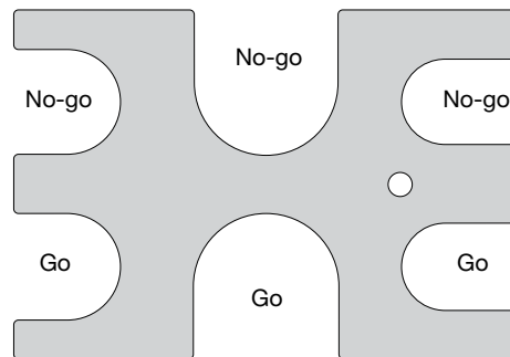
Crimp Gauge
