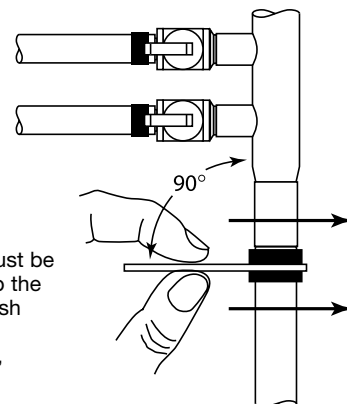
Crimp Gauge
