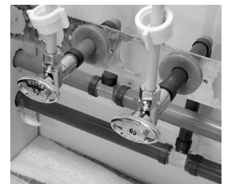
PEX Stubouts and Bracket/Grommets
