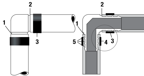
Illustration of a Good CrimpRing™ Connection
