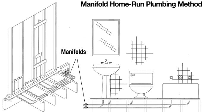
Manifold Home-Run Plumbing Method
