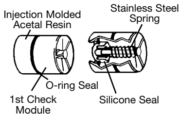
CHECK ASSEMBLY \frac{1}{4} " - \frac{3}{4} "
