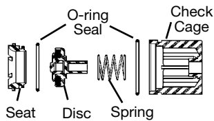
CHECK ASSEMBLY \frac{3}{4} " M3
