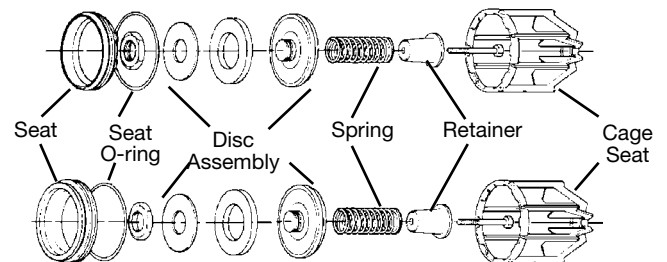
CHECK ASSEMBLY 2\frac{1}{2} " - 3"
