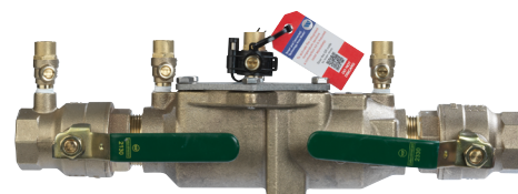
LF007 with freeze sensor
