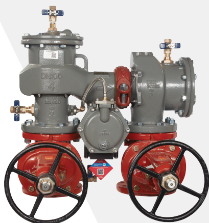
LF880V with flood sensor
