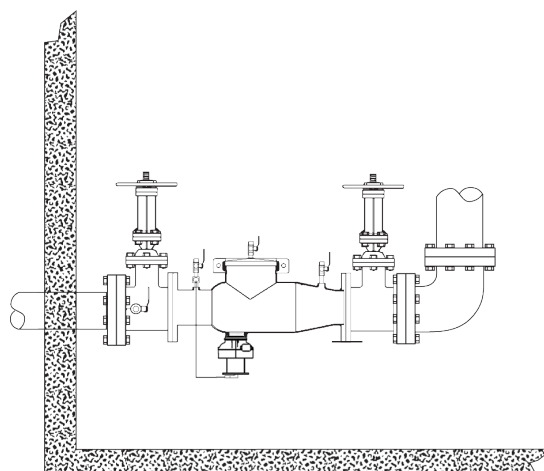
Outdoor Installation
