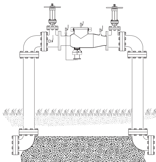
Outdoor Installation
