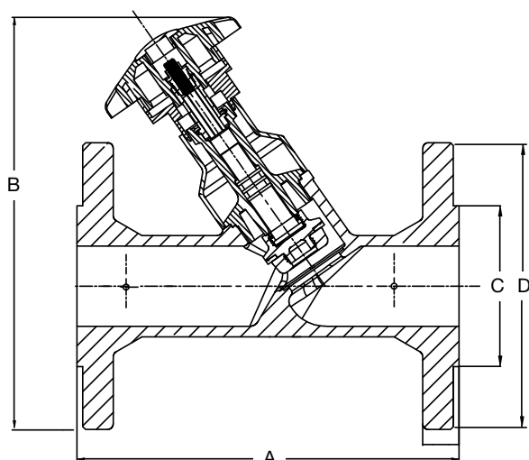
1 1/4" - 2" CSM-82-F
