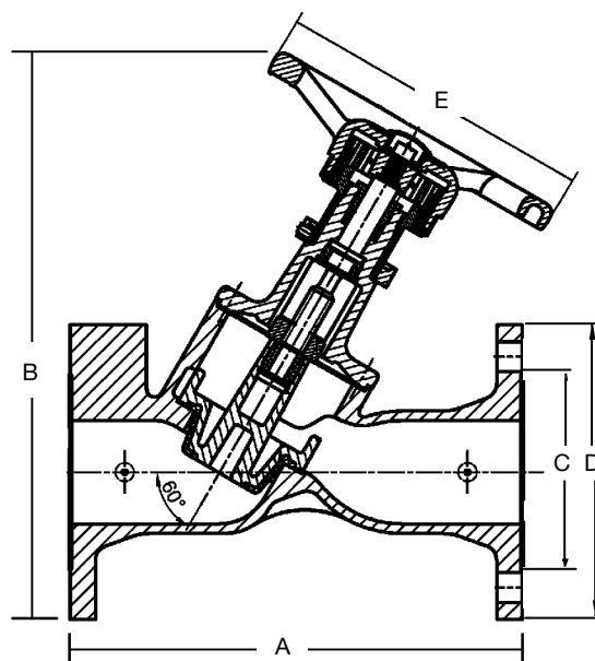
2 1/2" - 12" CSM-82-F
