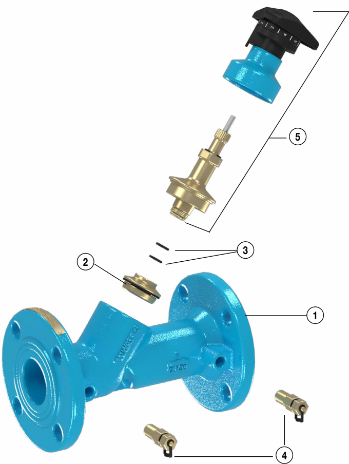
1 1/4" - 2" CSM-82-F
