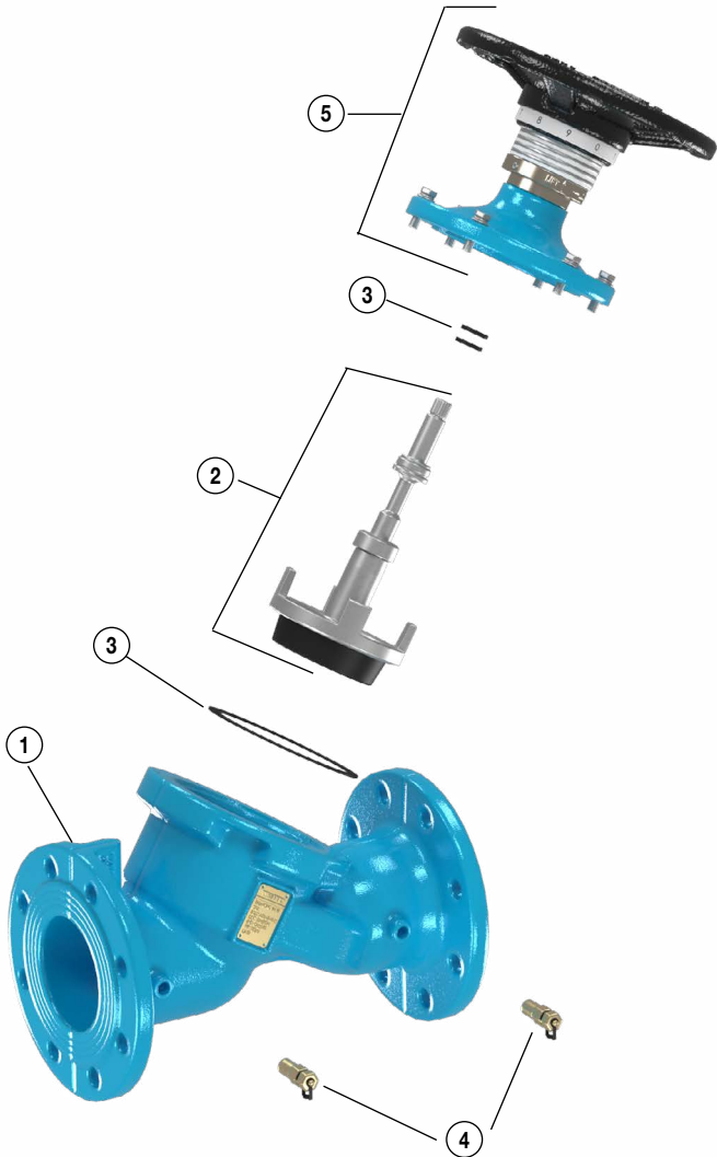
2 1/2" - 12" CSM-82-F
