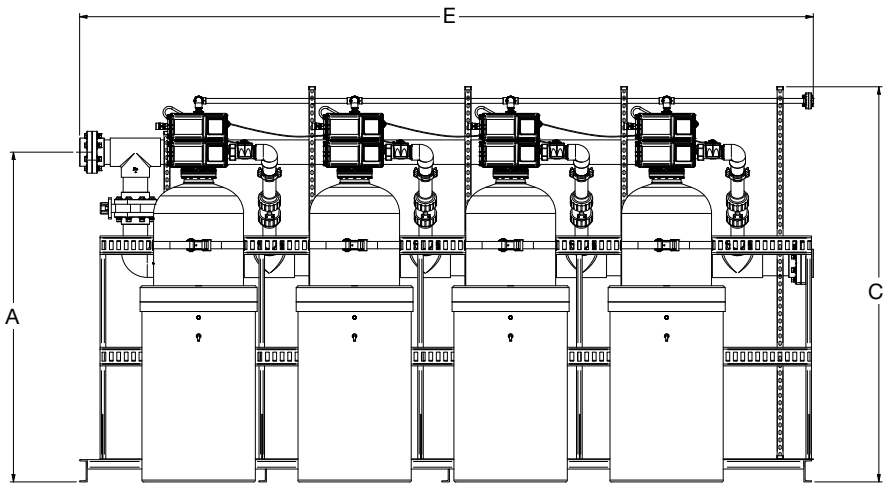
Front
