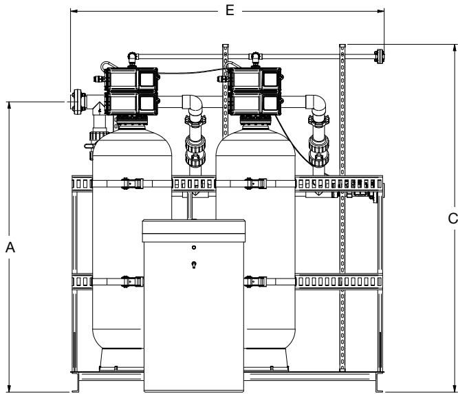
Front
