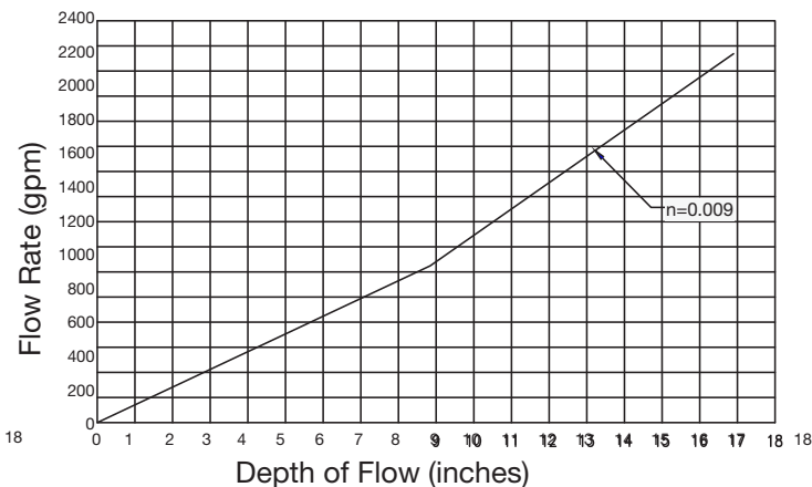
DLX 12" FLOW
